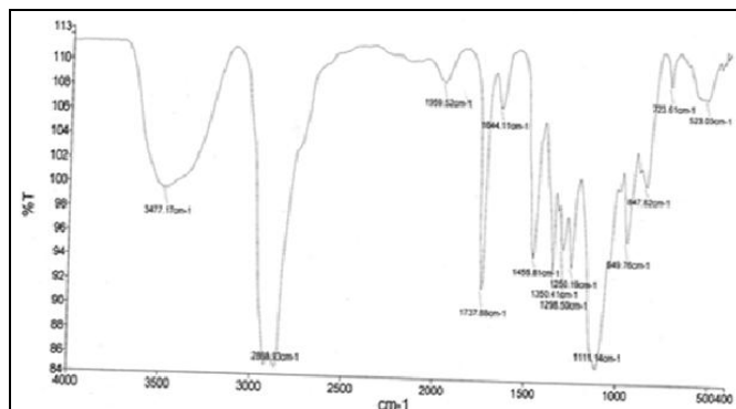
FIG. 3: FTIR SPECTRA OF POLYMER
